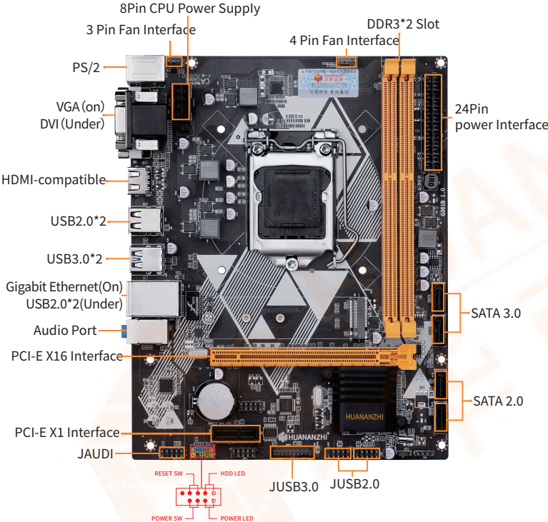
1-1 B85 MotherBoard Illustration
