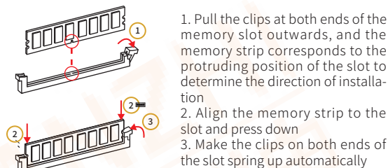
2-8 Memory Installation
