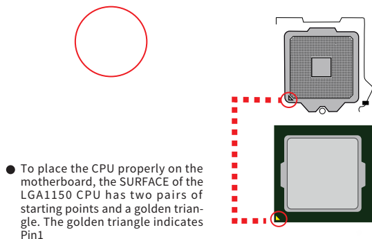
Figure 2-6 CPU installation
