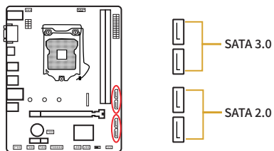
2-10 SATA Interface
