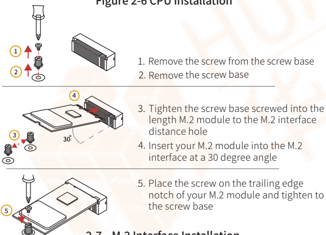
2-7 M.2 Interface Installation
